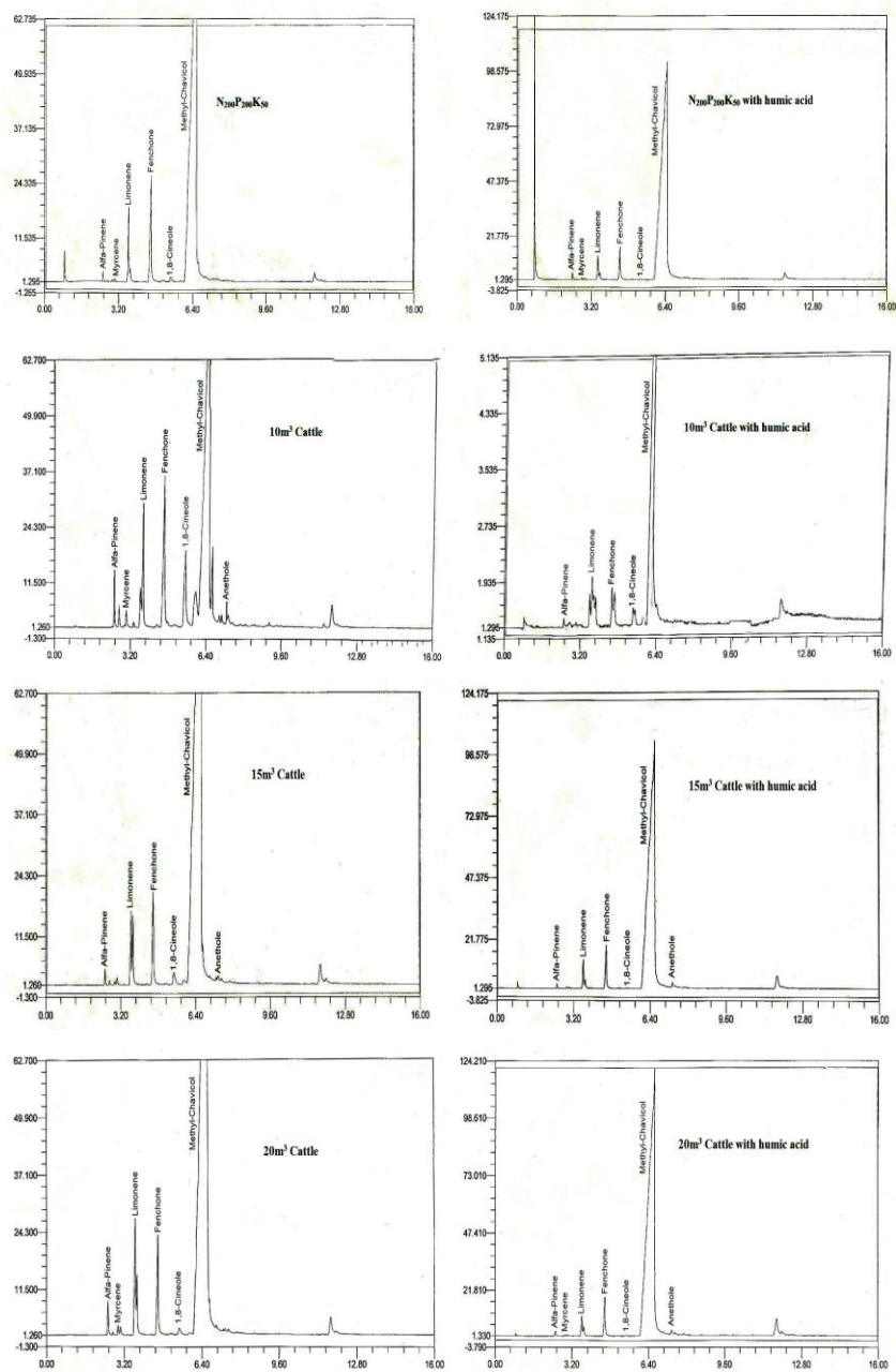
Fig. (2): G.L.C. chromatographic analysis of fennel oil components % from N 200 P 200 K 50 kg/fed and cattle manure at (10, 15 and 20 m 3 / fed) with or without humic acid application.
