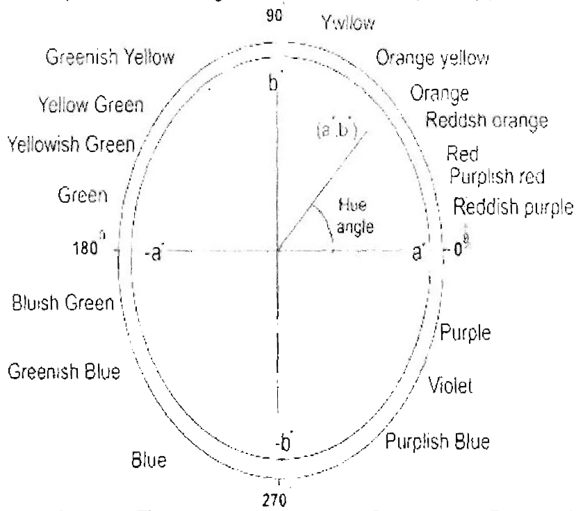
Picture (1): Hue sequence and hue-angle attenuation on a CIELAB diagram (with ISCC-NBS color names).
