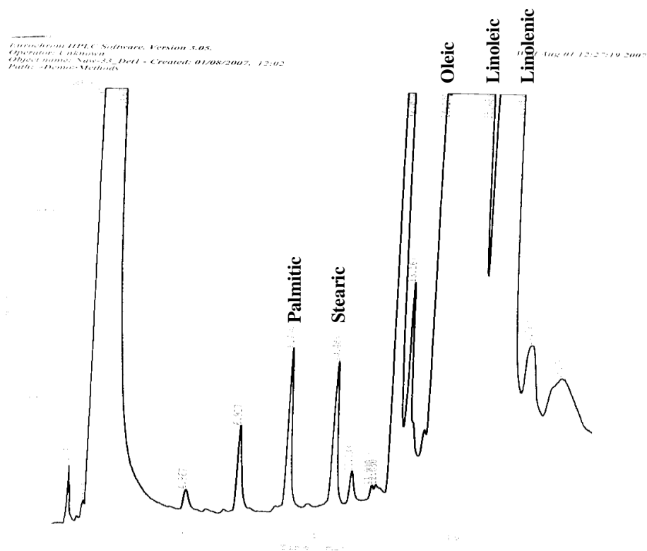
Fig (3): Main fatty acids of S. 2465/1 var. oil.
