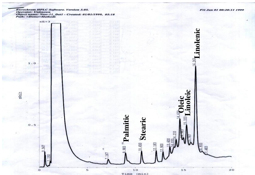
Fig (1): Main fatty acids of Sakha 1 var. oil.
